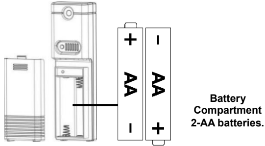
TX141-Bv2 Outdoor Sensor
